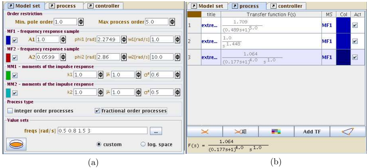
Fig. 3.4: a) Model set tab, b) Process tab.
